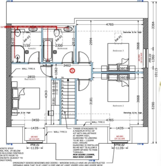
Proposed First Floor Plan 1:50
