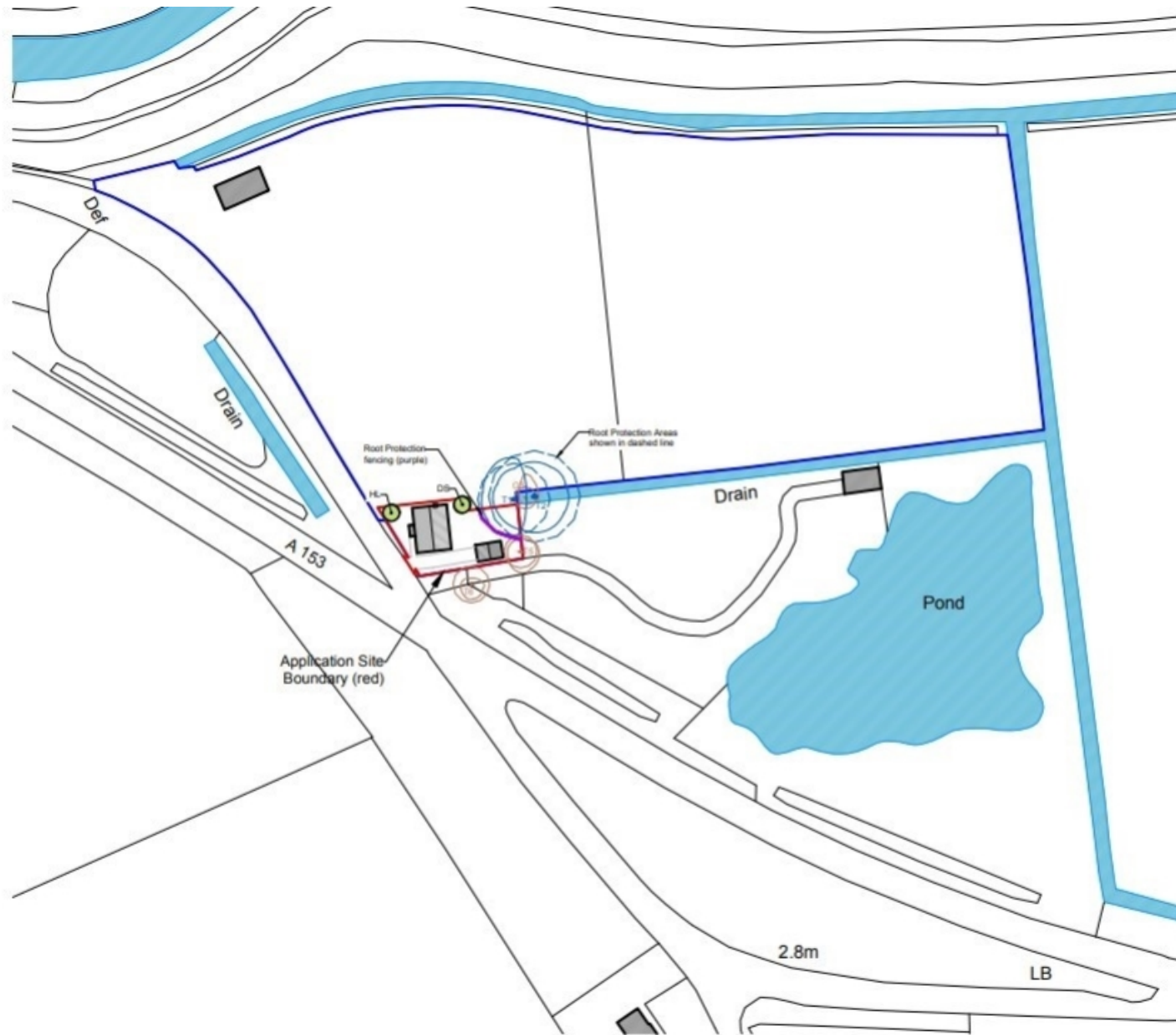
Proposed Site Location Plan
